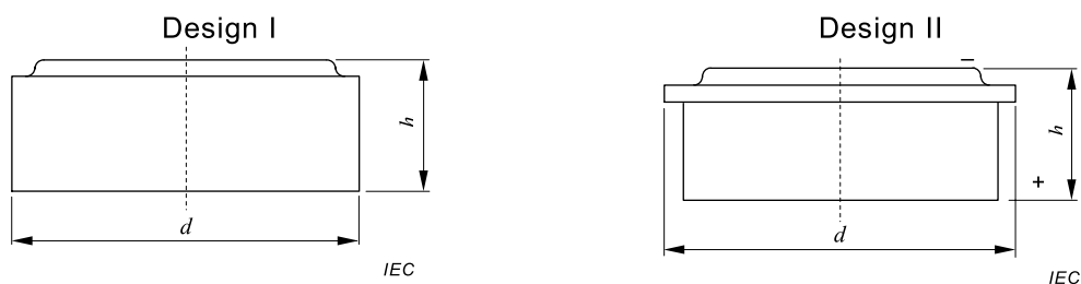
Figure 4 – Button cells
